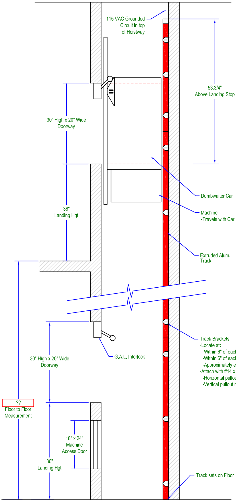
Side View of Hoistway
